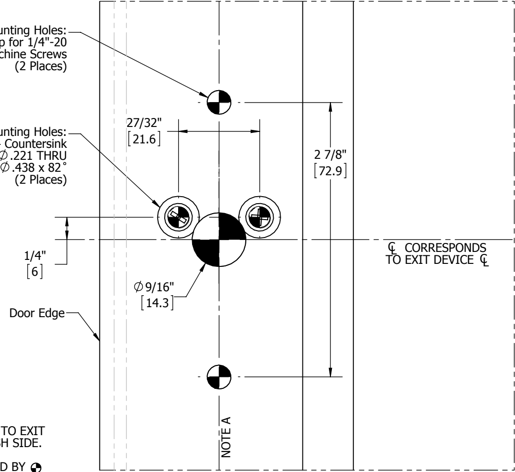
PUSH SIDE OF DOOR (EXIT DEVICE IS MOUNTED ON THIS SIDE)
