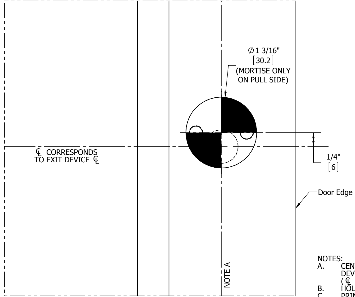
PULL SIDE OF DOOR (RIM CYLINDER IS MOUNTED ON THIS SIDE)
