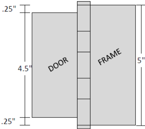
UNEQUAL LEAF CENTERED (RH standard)
